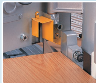
End cutting of front and back of the tape.
